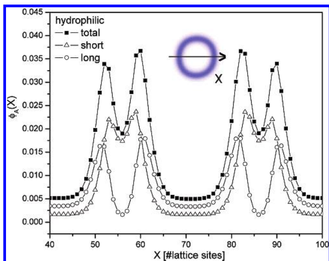
Figure 4. Density distribution of a large size vesicle with hydrophilic block PI = 1.33 and \chi_{AB}\bar{N} = 31.3 .
